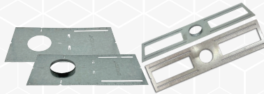
PLATE13-3A | PLATE13-3A-L | PLATE26-3A | PLATE26-3A-L Construction plate made up of galvanized steel for recessed lighting
