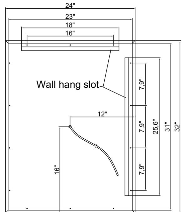
REAR VIEW
