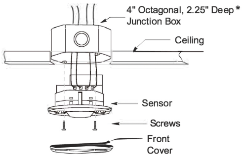
Mounting to an Octagonal Junction Box
